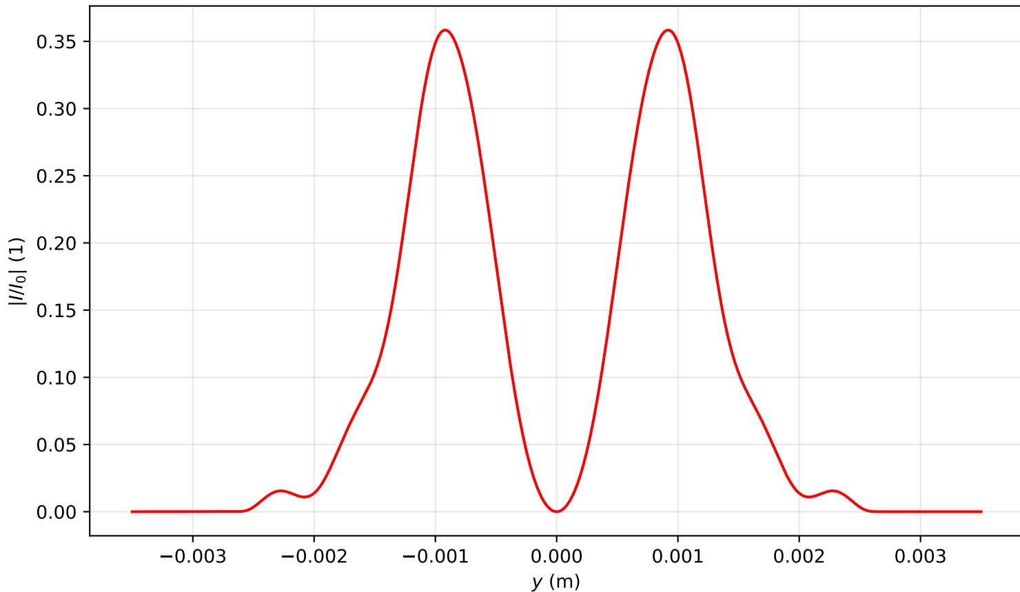
Intensity profile I(x=0, y, z=3.742)/I_0 , P_{in}=3.0P_{cr} , artificial time
